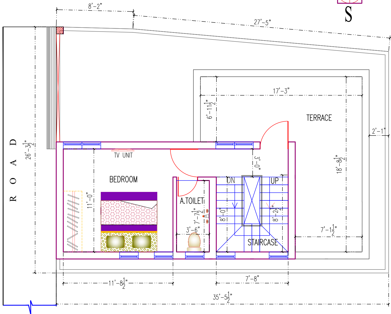
FIRST FLOOR
