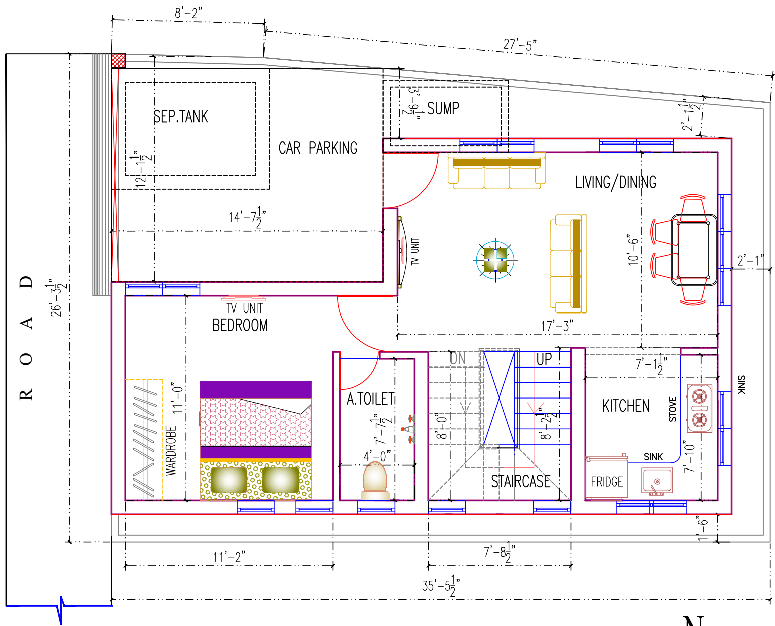
GROUND FLOOR
